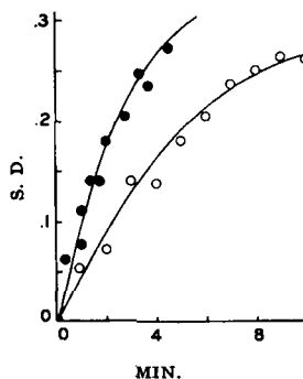
Fig. 1.—Plot of the standard deviation of a binary system vs. time of agitation. Solid points are at a 1:1 weight ratio of 8/32 vs. 3/32 in. steel balls. Open points are at a 1:1 weight ratio of 6/32 vs. 3/32 in. steel balls.
